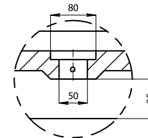
DETAIL D SCALE 1:3
