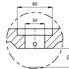
DETAIL D SCALE 1:4
